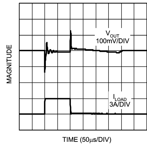
Load Transient Response (Tantalum 100 \mu\text{F}/3\text{A} )
