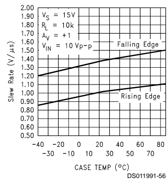
Slew Rate vs Temperature
