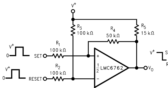
FIGURE 7. Bi-Stable Multivibrator
