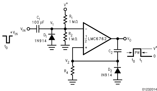
FIGURE 6. One-Shot Multivibrator
