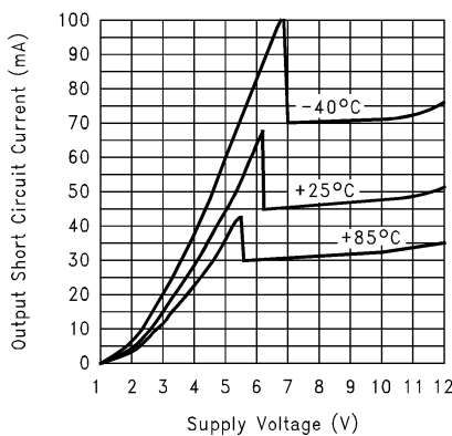
Output Short Circuit Current vs Supply Voltage (Sinking)
