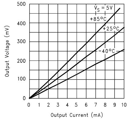
Output Voltage vs Output Current (Sinking)
