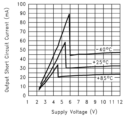
Output Short Circuit Current vs Supply Voltage (Sourcing)
