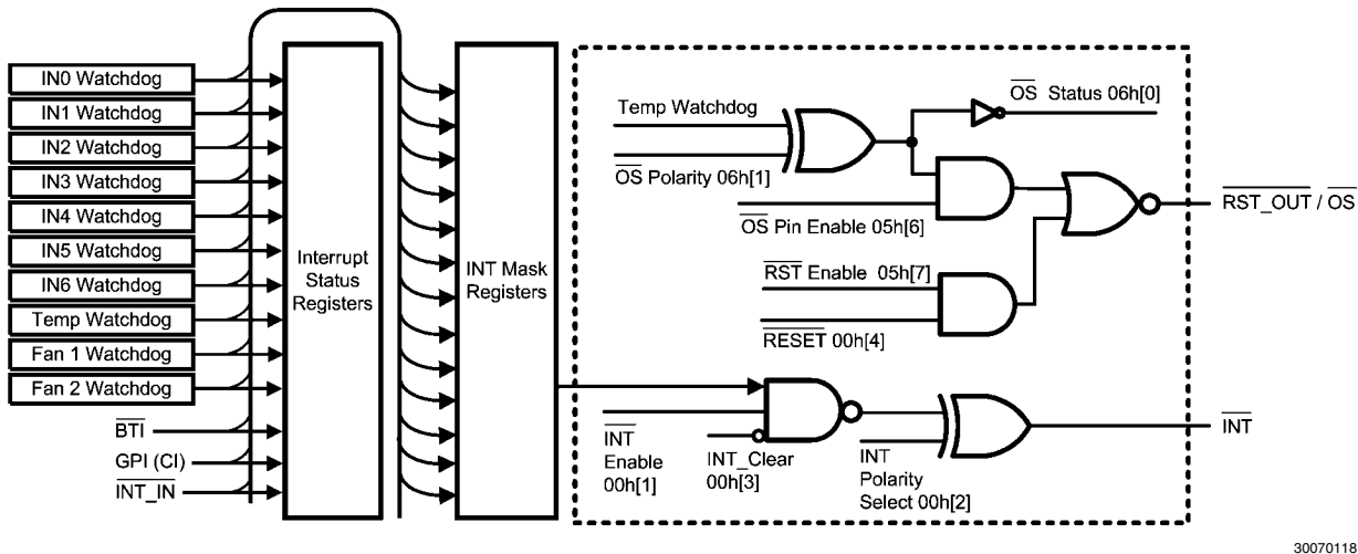
FIGURE 8. Interrupt Structure
