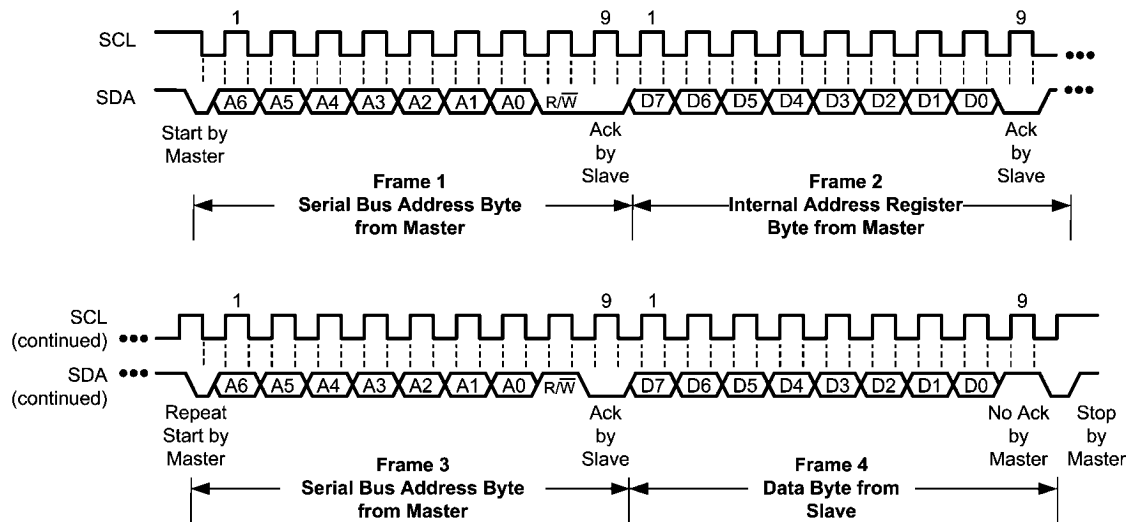
(e) Single Byte Read from Register with Internal Address Set using a Repeat Start
