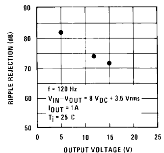
Ripple Rejection
