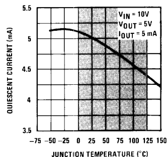
Quiescent Current
