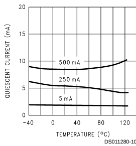
Quiescent Current vs Temperature
