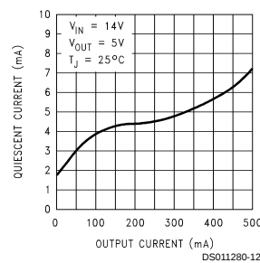
Quiescent Current vs Output Current
