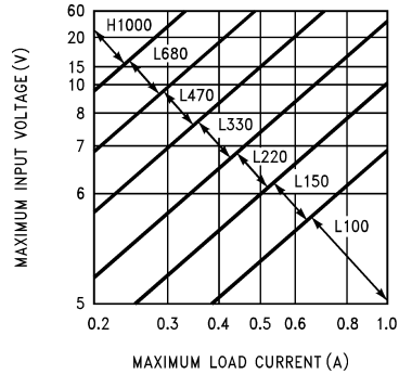
FIGURE 3. LM2575(HV)-3.3
