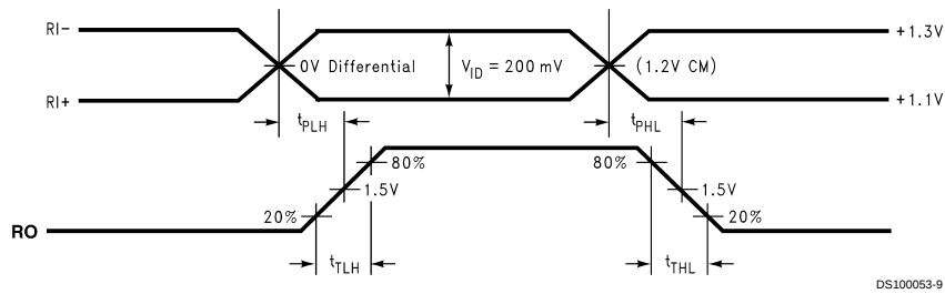
FIGURE 7. Receiver Propagation Delay and Transition Time Waveforms
