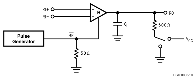
FIGURE 8. Receiver TRI-STATE Delay Test Circuit
