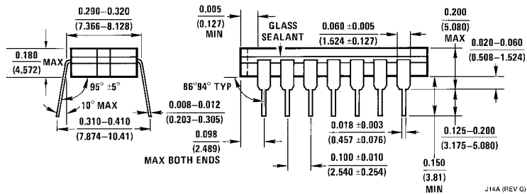
14-Lead Ceramic Dual-In-Line Package (J) Order Number 54LS00DMQB or DM54LS00J Package Number J14A
