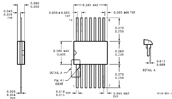
14-Lead Ceramic Flat Package (W) Order Number 54LS00FMQB or DM54LS00W Package Number W14B
