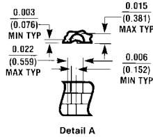
Ceramic Leadless Chip Carrier Package (E) Order Number 54LS00LMQB Package Number E20A
