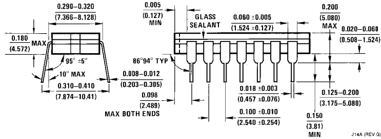
14-Lead Ceramic Dual-In-Line Package (J) Order Number DM5407J NS Package Number J14A
