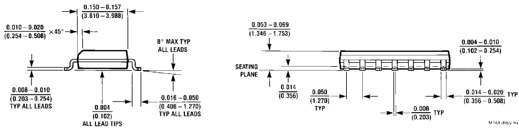
14-Lead Small Outline Molded Package (M) Order Number DM7407M NS Package Number M14A
