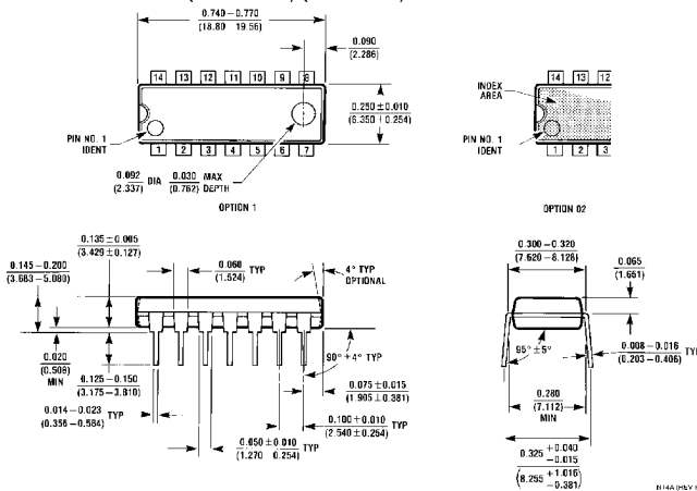
14-Lead Molded Dual-In-Line Package (N) Order Number DM7407N NS Package Number N14A
