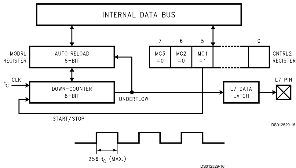
FIGURE 13. Mode 2a: 50% Duty Cycle Output
