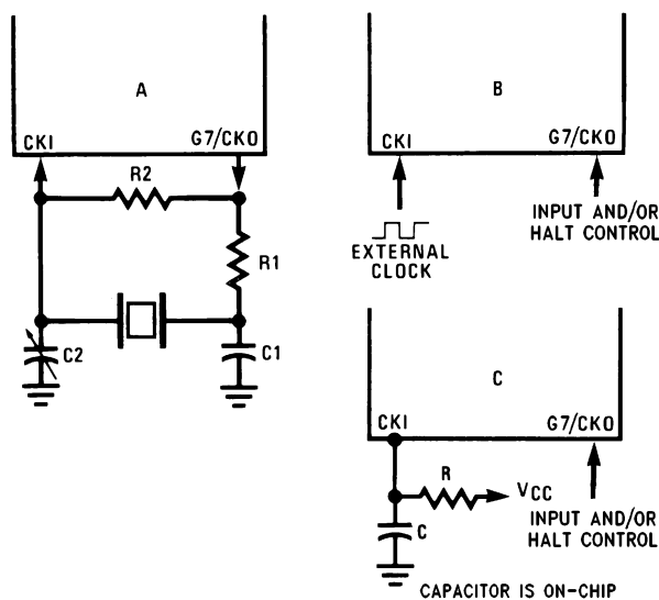
FIGURE 5. Clock Oscillator Configurations
