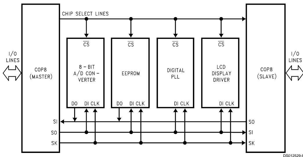
FIGURE 7. MICROWIRE/PLUS Application
