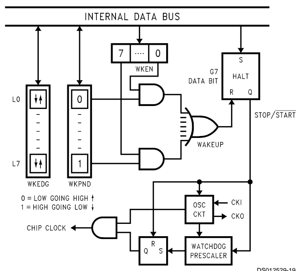
FIGURE 15. Multi-Input Wakeup Logic
