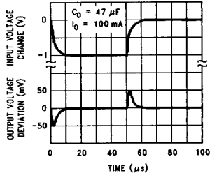
LM2990-12 and LM2990-15 Load Transient Response
