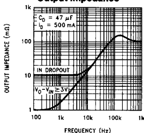
LM2990-5 and LM2990-5.2 Output Impedance
