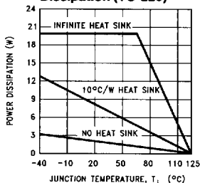
Maximum Power Dissipation (TO-220)
