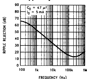
LM2990-12 and LM2990-15 Ripple Rejection
