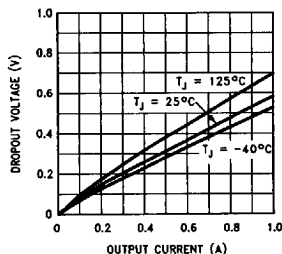
Dropout Voltage
