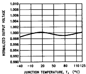
Normalized Output Voltage
