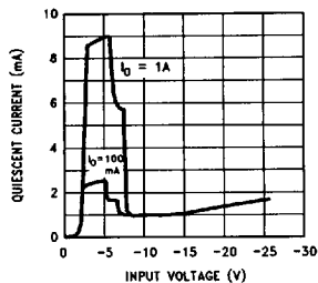
LM2990-5.0 and LM2990-5.2 Quiescent Current
