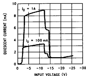
LM2990-12 Quiescent Current
