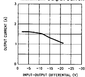
Maximum Output Current
