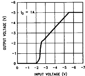
LM2990-5 and LM2990-5.2 Low Voltage Behavior
