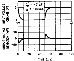
LM2990-5 and LM2990-5.2 Line Transient Response
