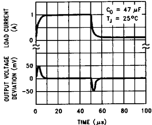
LM2990-5 and LM2990-5.2 Load Transient Response
