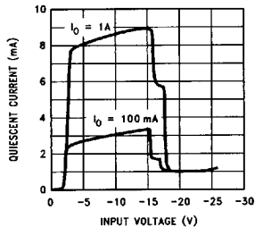
LM2990-15 Quiescent Current
