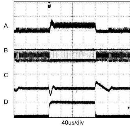
Load Transient Response (PWM Mode)
