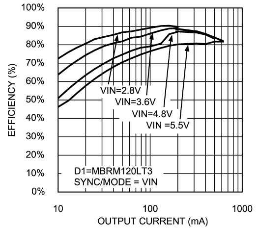
Efficiency vs Output Current ( V_{OUT} = 1.5V , PWM Mode, With Diode)
