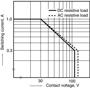
1. Max. switching capacity
