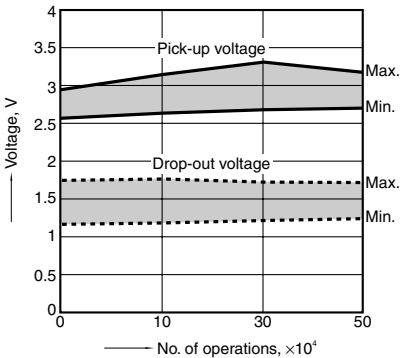
3. Mechanical life
