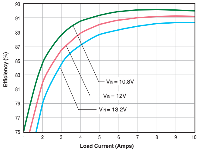
LSM-2/10-D12 Efficiency vs. Line Voltage and Load Current @ +25°C
