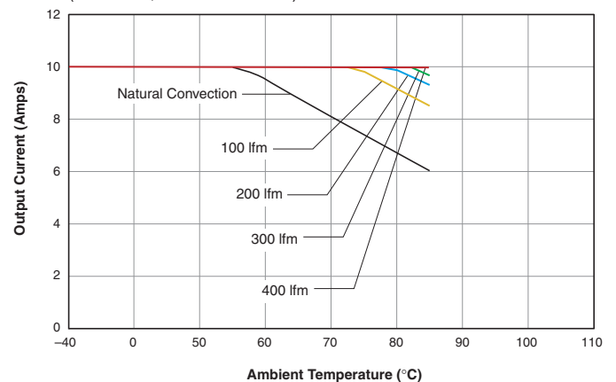
LSM-T/10-D12 Maximum Output Current vs. Ambient Temperature (V OUT = 5V, transverse airflow)
