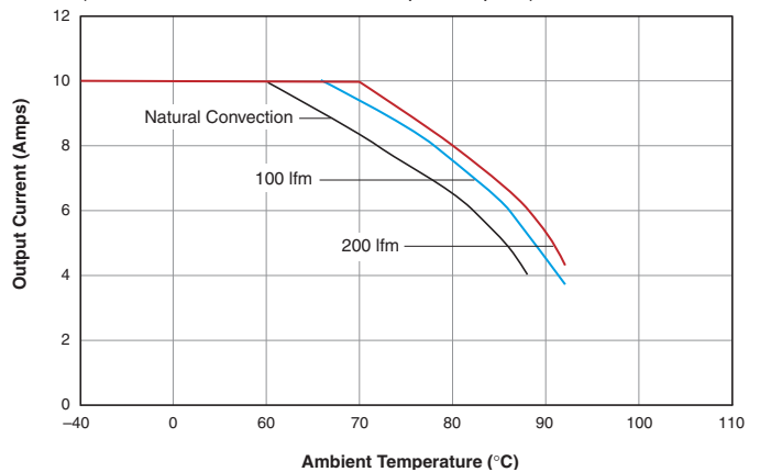
LSM-1.5/10-D12 Maximum Output Current vs. Ambient Temperature (SMTmount, air flow direction from pin 2 to pin 1)
