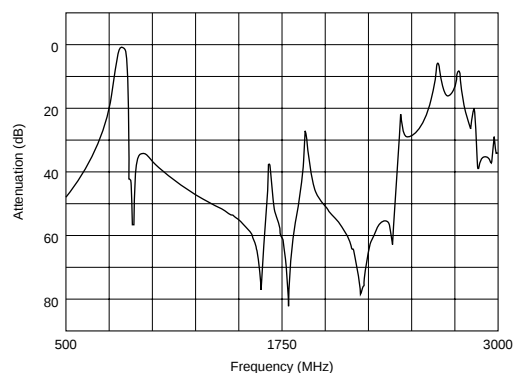
Spurious (Tx)
