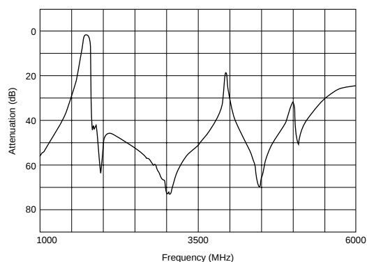
Spurious (Tx)
