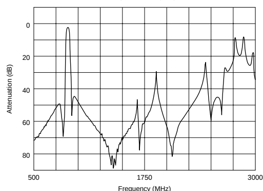
Spurious (Rx)
