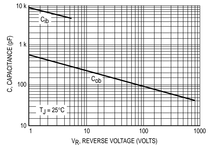
Figure 6. Capacitance
