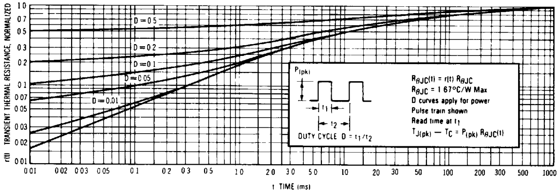
Figure 10. Thermal Response
