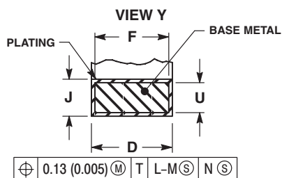
SECTION AB-AB ROTATED 90° CLOCKWISE
