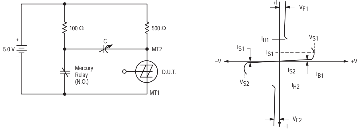
FIGURE 9 – TURN-OFF TIME TEST CIRCUIT
