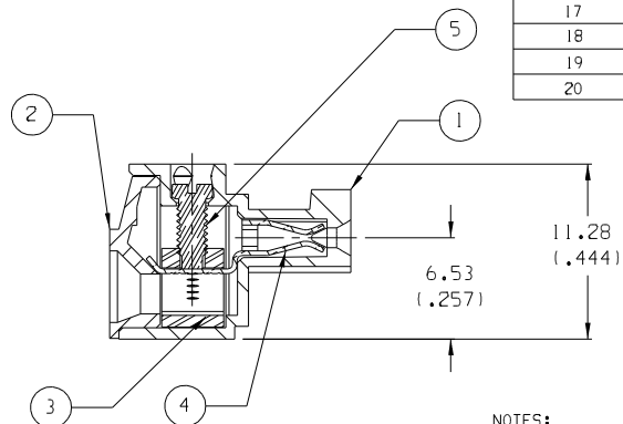
SECTION Z-Z
