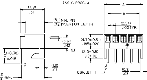
RECOMMENDED P.C. BOARD LAYOUT FOR ASS'Y. PROC. A
