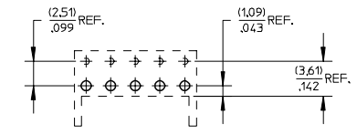
RECOMMENDED P.C. BOARD LAYOUT FOR ASS'Y. PROC. C
