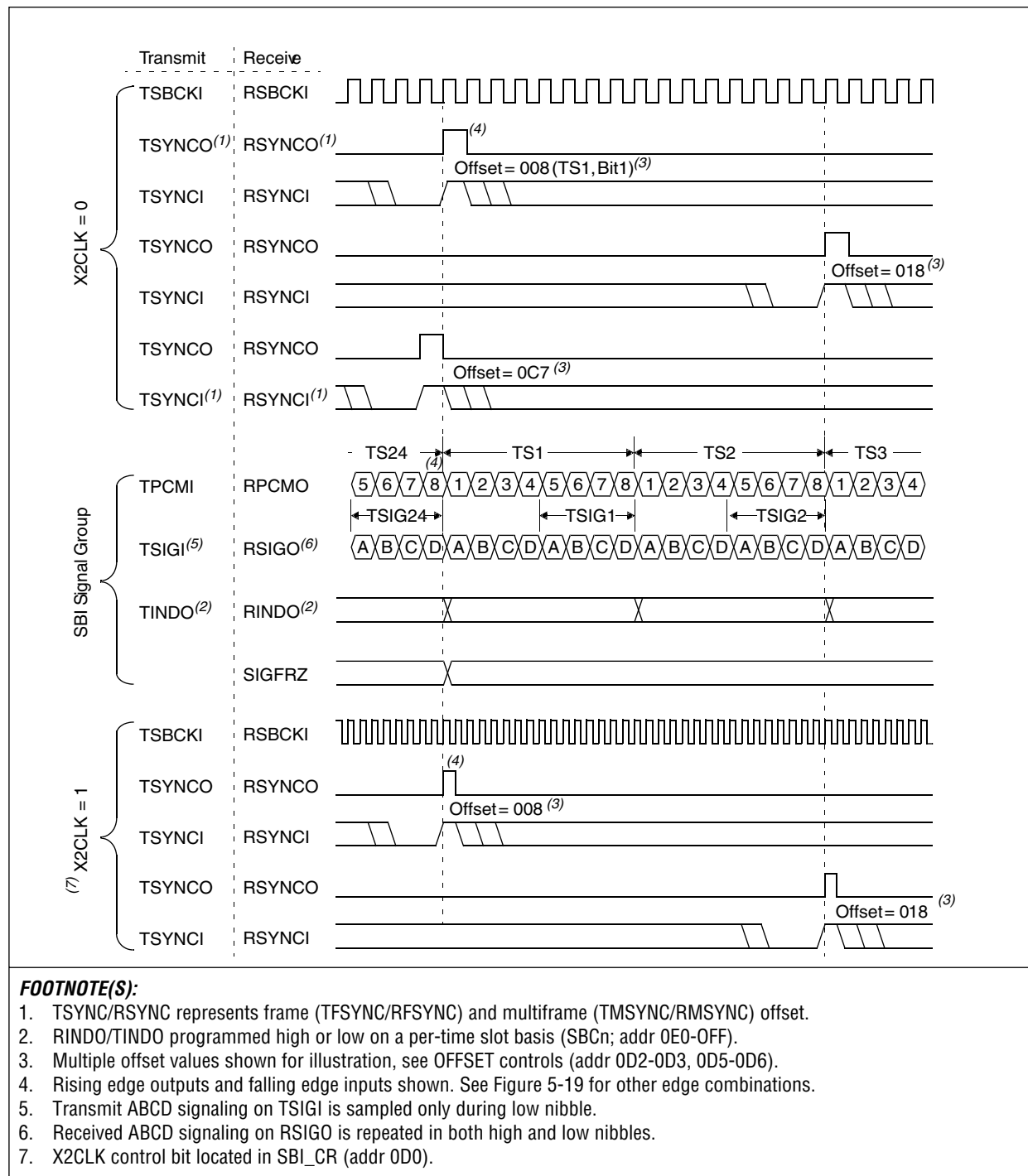
Figure 5-14. SBI Timing—1536K Mode
