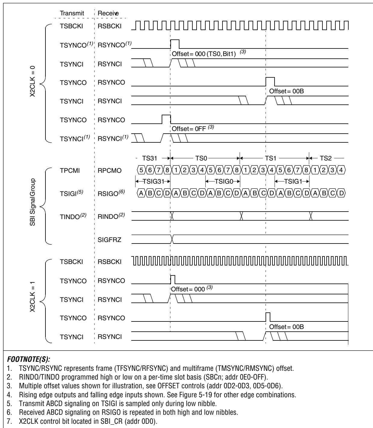
Figure 5-16. SBI Timing—2048K Mode
