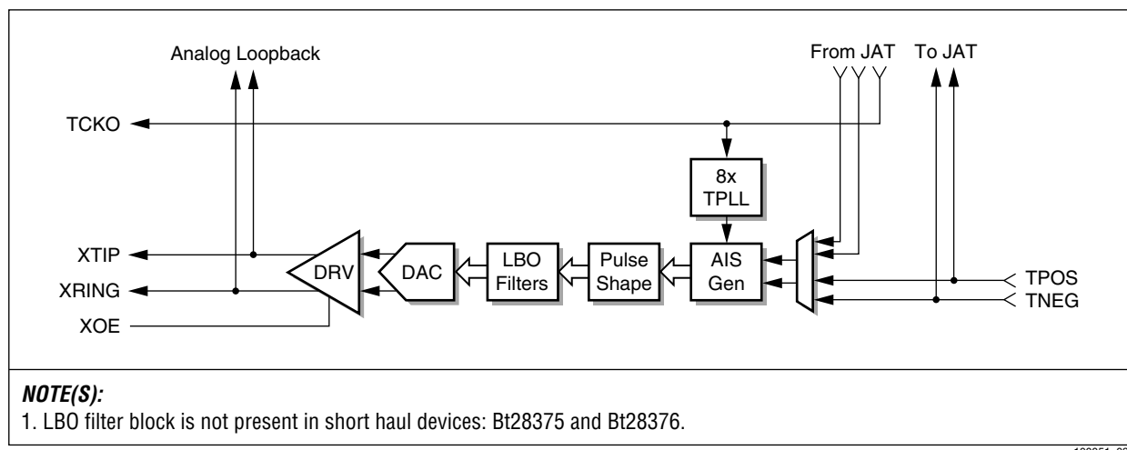
Figure 2-33. TLIU Diagram
