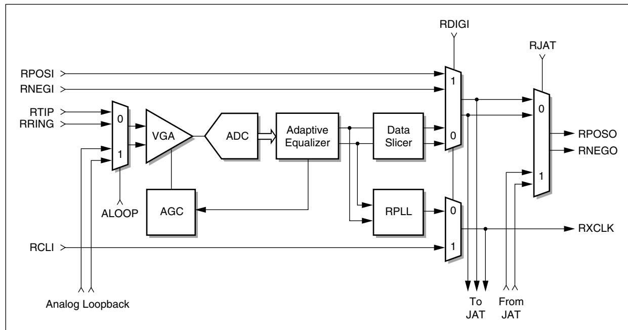
Figure 2-4. RLIU Diagram
