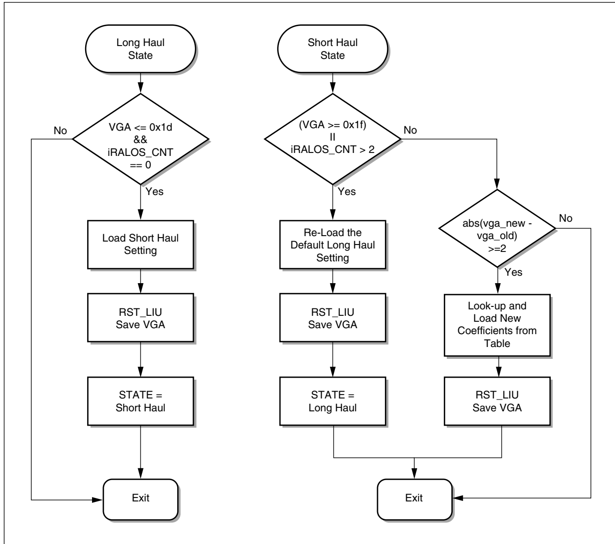
Figure D-4. The Short Haul and Long Haul State for E1-75 Interface
