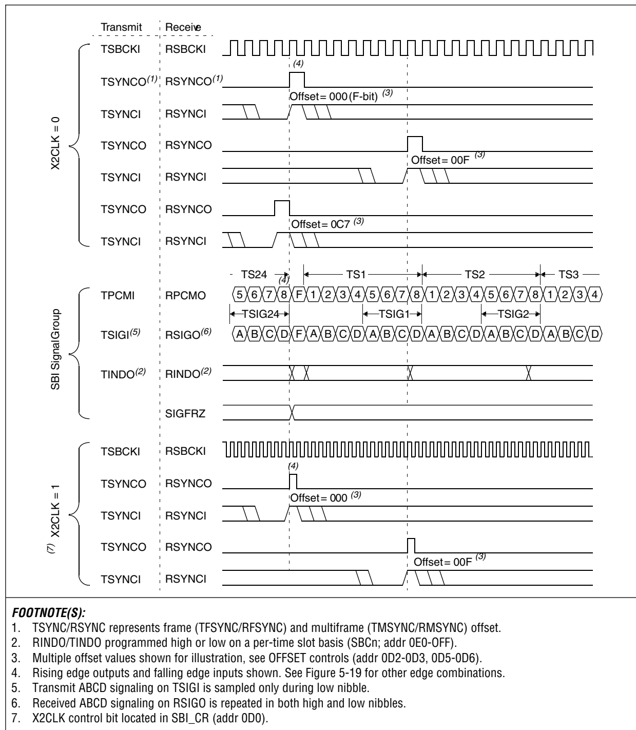
Figure 5-15. SBI Timing—1544K Mode
