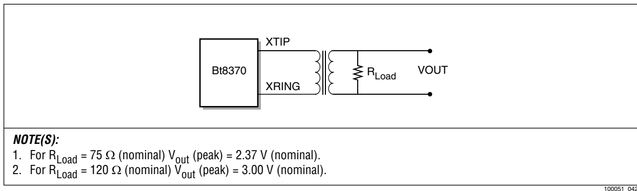
Figure 2-38. E1 (G.703) Pulse Template Test Circuit
