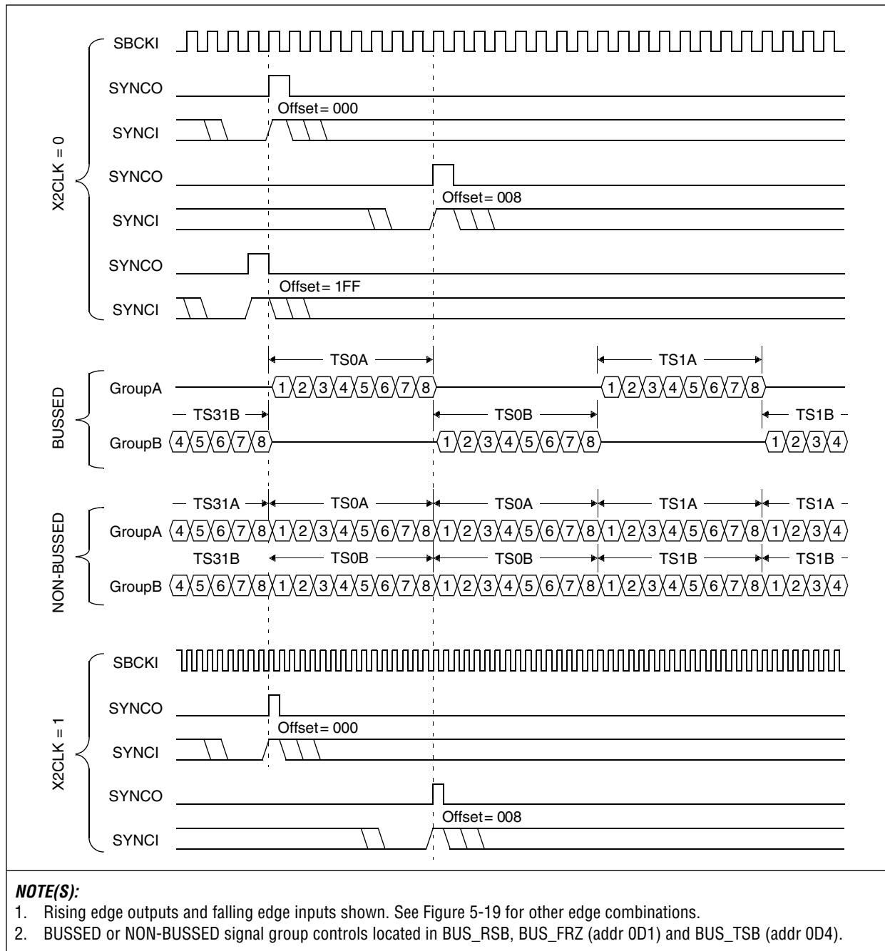
Figure 5-17. SBI Timing—4096K Mode
