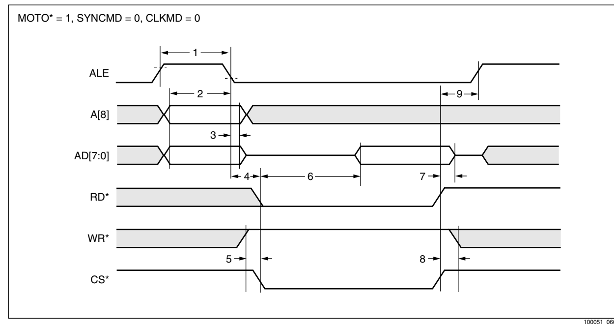
Figure 5-8. Intel Asynchronous Read Cycle
