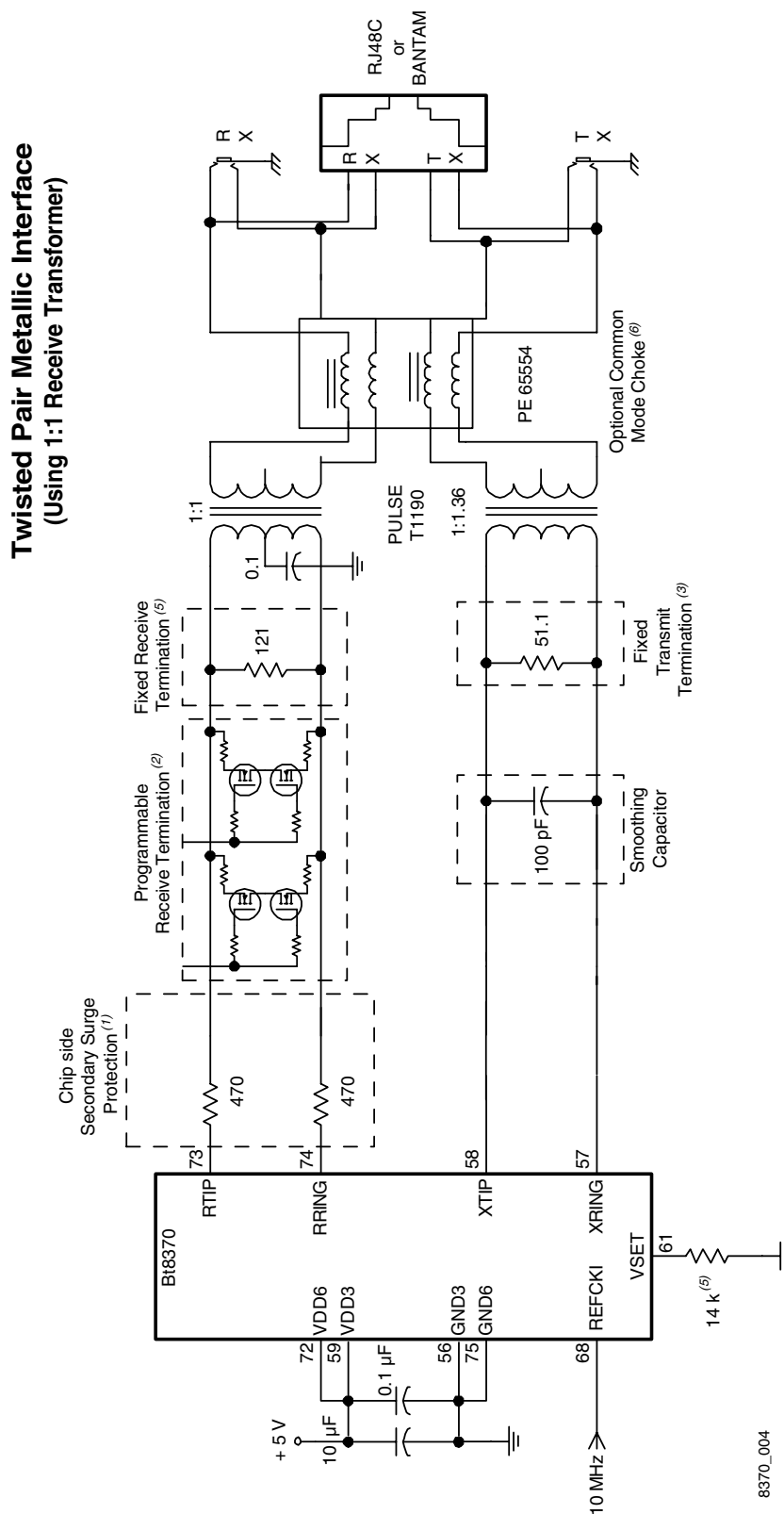
Figure 4-4. Option D: Short Haul Application (1 of 2)
