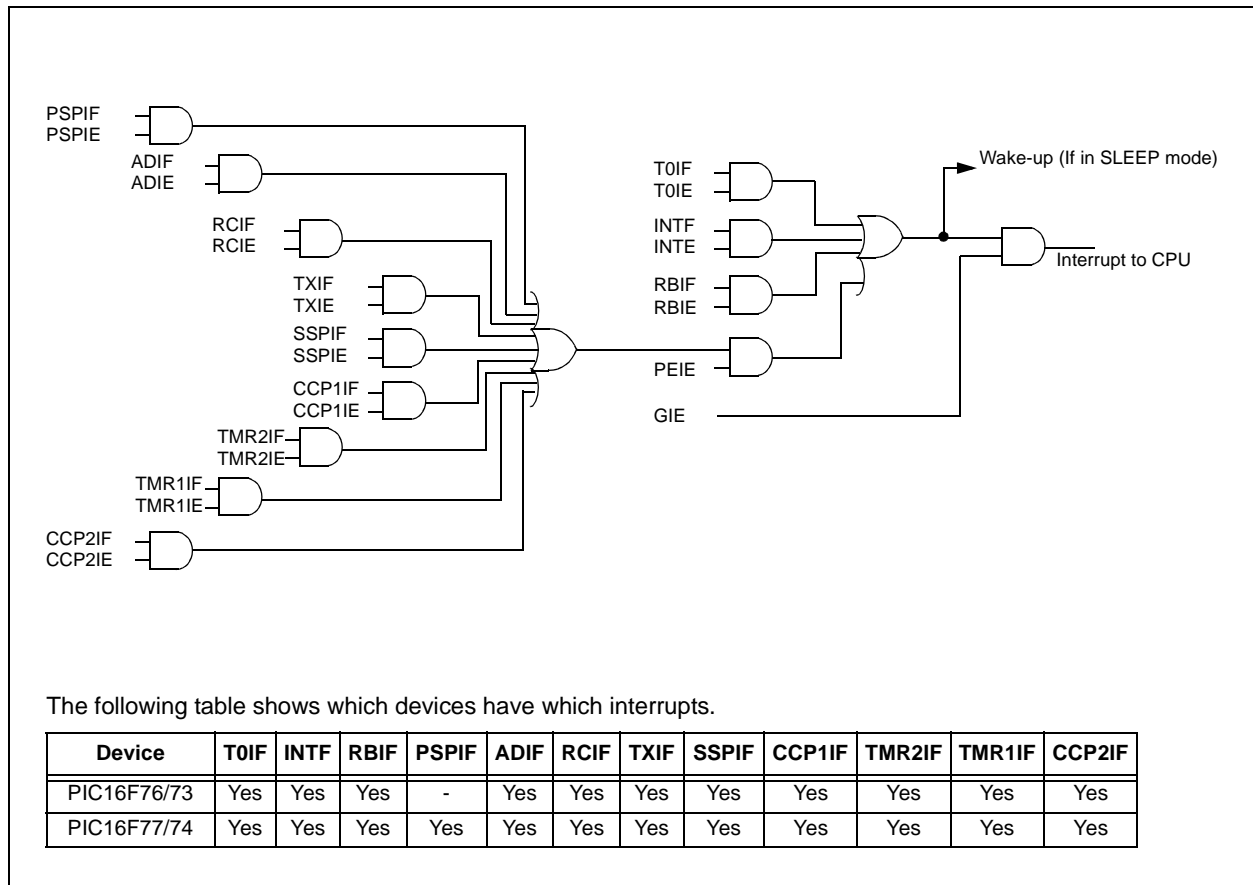
FIGURE 12-9: INTERRUPT LOGIC
