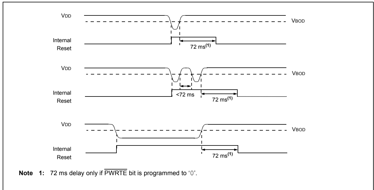
FIGURE 9-6: BROWN-OUT SITUATIONS
