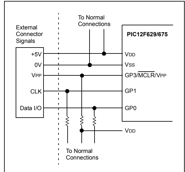
FIGURE 9-14: TYPICAL IN-CIRCUIT SERIAL PROGRAMMING CONNECTION
