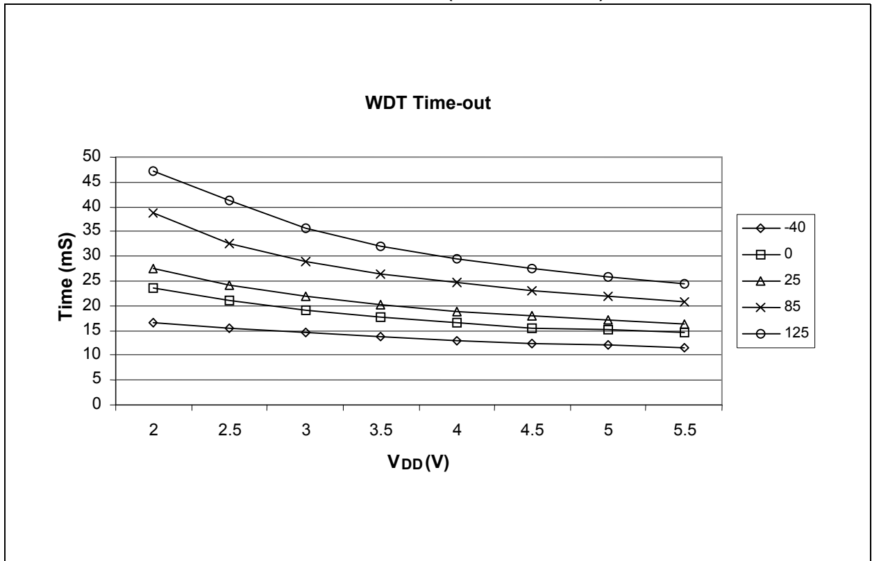
FIGURE 13-17: TYPICAL WDT PERIOD vs. V_{DD} ( -40^{\circ}\text{C} TO +125^{\circ}\text{C} )
