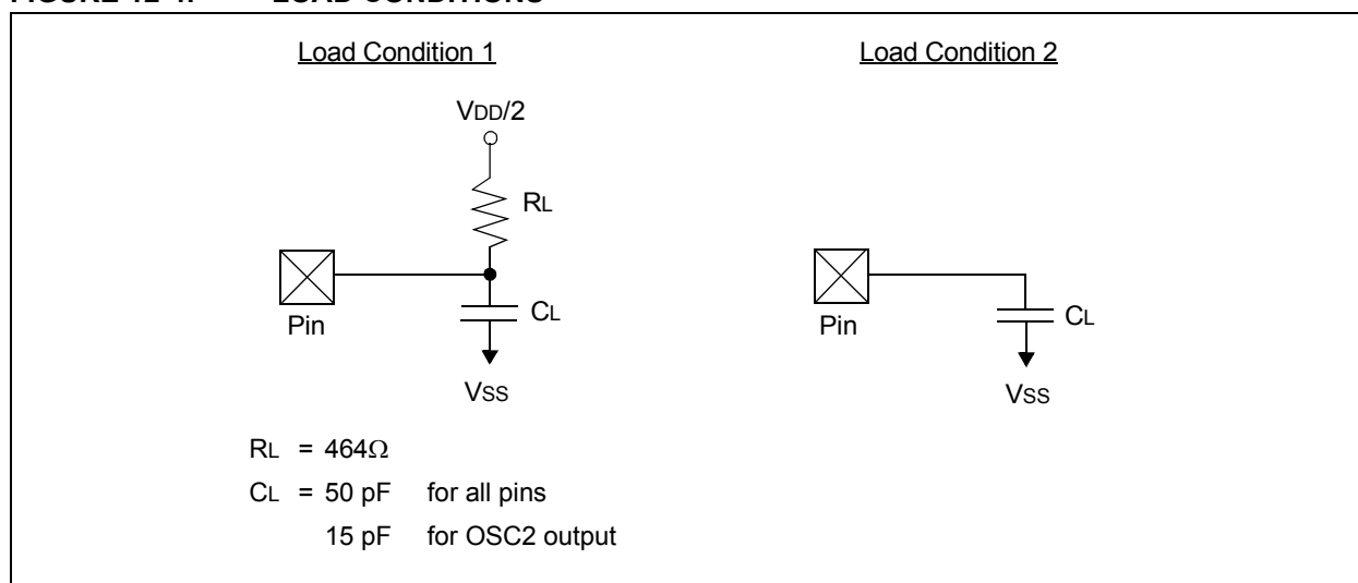
FIGURE 12-4: LOAD CONDITIONS
