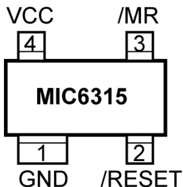
4-Pin SOT-143 (U) (Top View)
