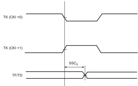
Figure 58-33. SSC Transmitter, TK and TF in Output
