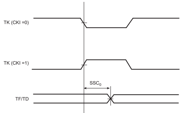
Figure 59-31. SSC Transmitter, TK and TF in Output
