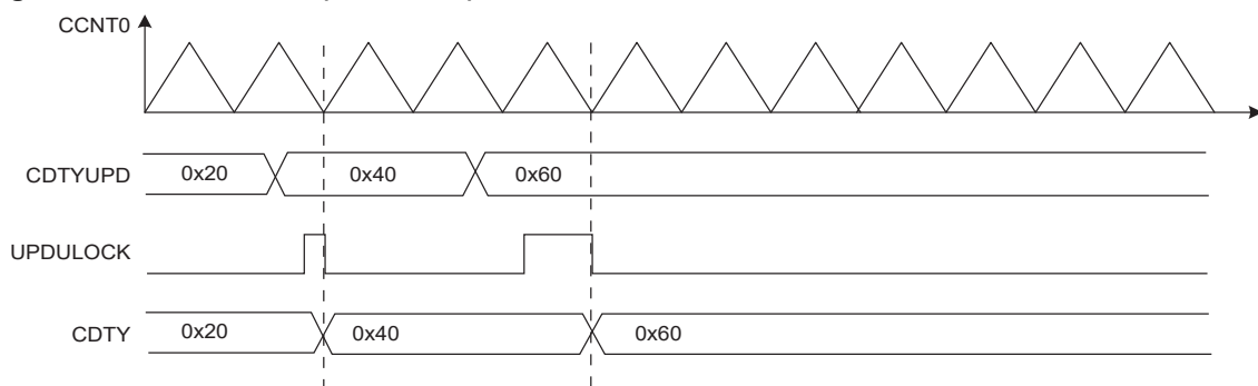
Figure 51-19. Method 1 (UPDM = 0)
