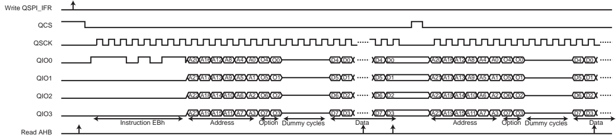
Figure 42-17. Instruction Transmission Waveform 7
