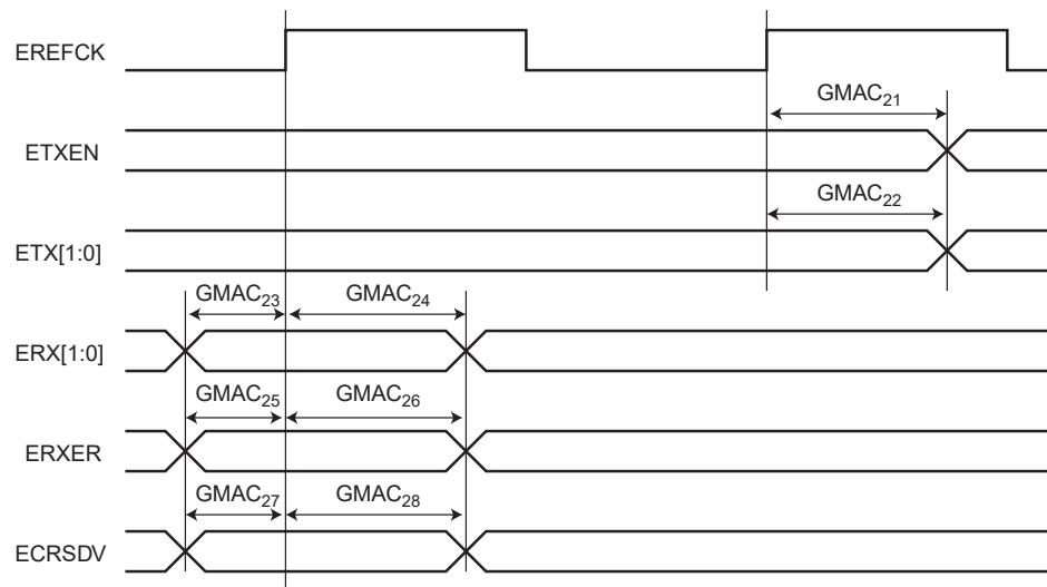
Figure 59-30. GMAC RMII Mode Signals
