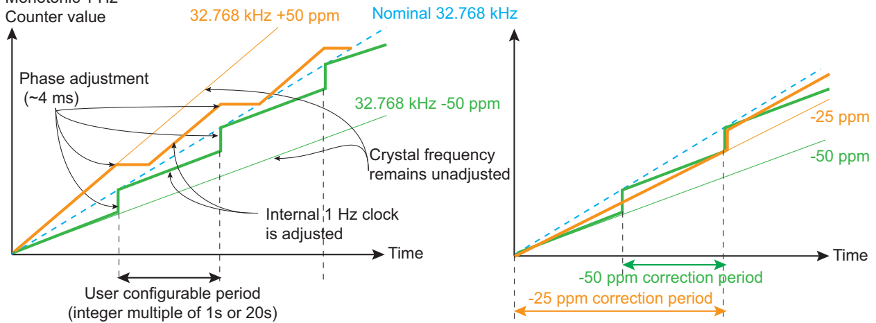
Figure 27-5. Calibration Circuitry Waveforms
