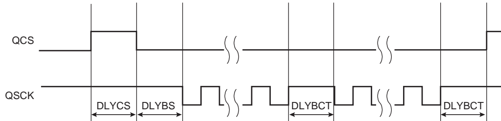
Figure 42-4. Programmable Delays
