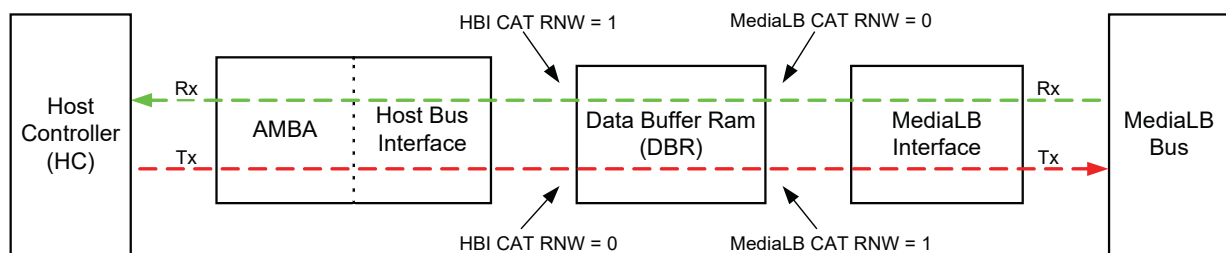
Figure 48-16. MLB DBR Directional Relationship
