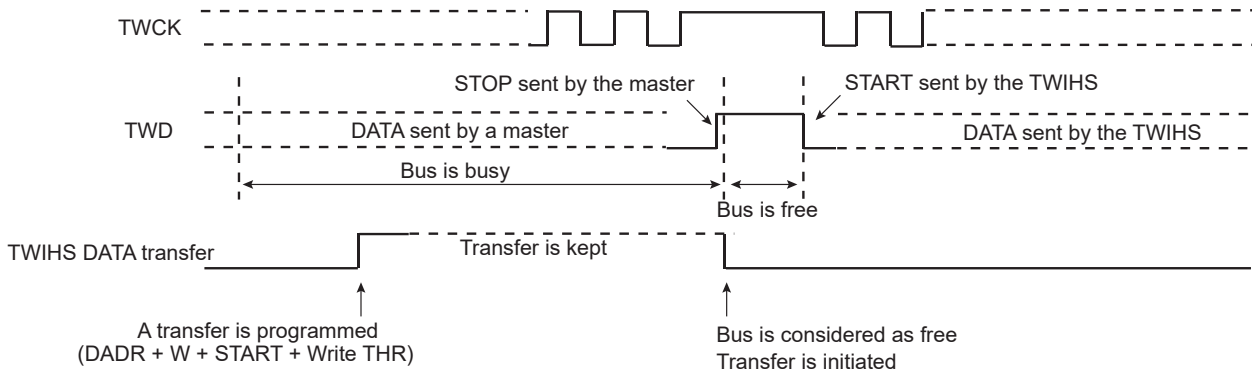
Figure 43-29. Arbitration Cases
