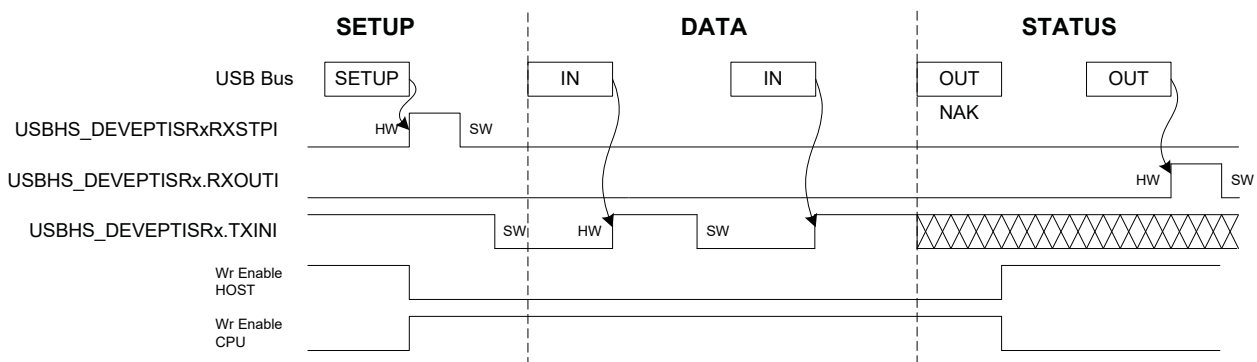
Figure 39-10. Control Read
