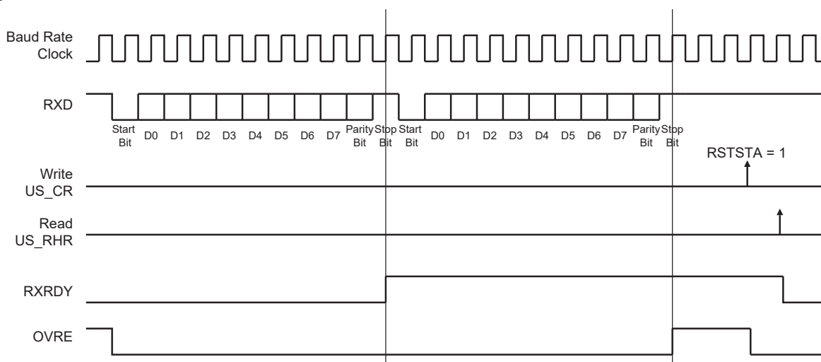
Figure 46-20. Receiver Status
