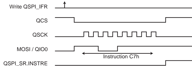
Figure 42-11. Instruction Transmission Waveform 1
