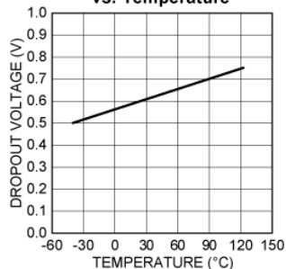
MIC2975x Dropout Voltage vs. Temperature
