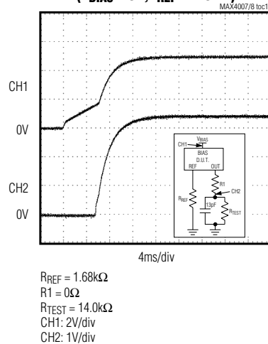
STARTUP DELAY ( V_{\text{BIAS}} = 5\text{V} , I_{\text{REF}} = 2.5\text{mA} )
