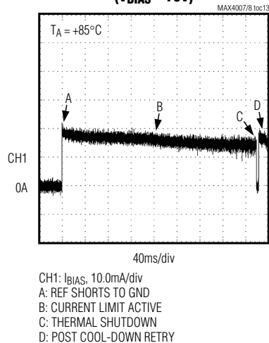
SHORT-CIRCUIT RESPONSE ( V_{\text{BIAS}} = 76\text{V} )
