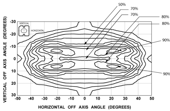
Figure 5b. HPWT-Rx00 Relative Luminous Intensity vs. Off Axis Angle. Iso-Intensity Contour Plot.
