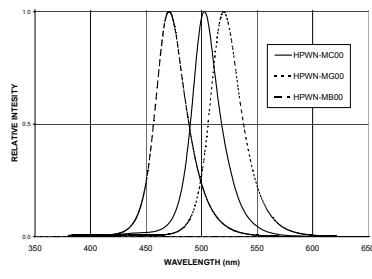
Figure 1b. Relative Intensity vs. Wavelength (HPWN)
