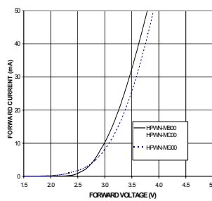
Figure 2b. Forward Current vs. Forward Voltage
