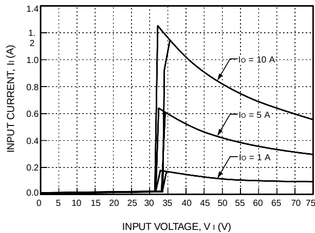
Figure 1. Typical JFW050F Input Characteristics at Room Temperature
