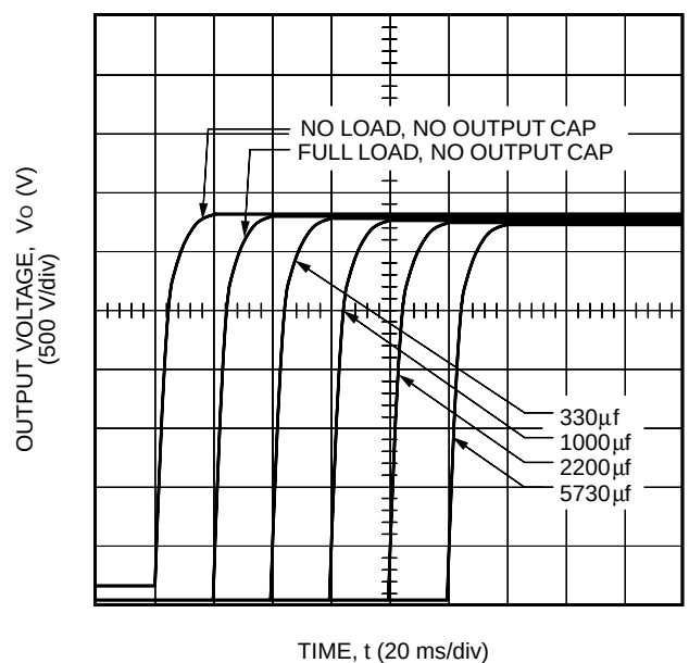
Figure 16. Typical Start-Up from Remote On/Off JFW150F1; Io = Full Load
