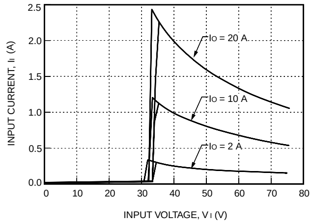
Figure 3. Typical JFW100F Input Characteristics at Room Temperature
