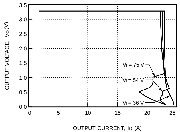
Figure 7. Typical JFW100F Output Characteristics at Room Temperature
