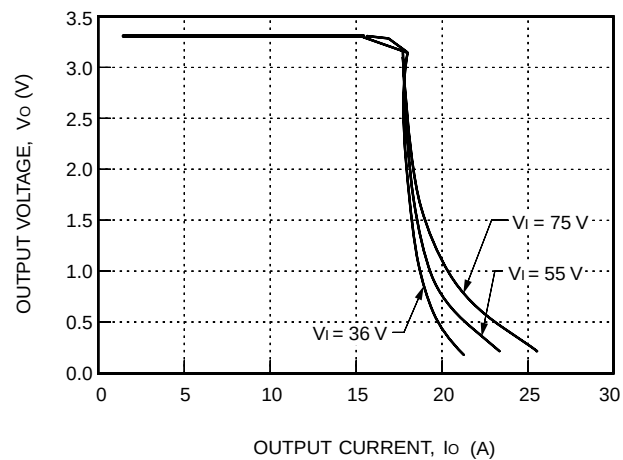
Figure 6. Typical JFW075F Output Characteristics at Room Temperature
