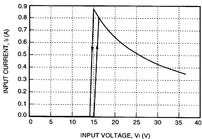
Figure 1. LC010 Input Current vs. Input Voltage at I o = I o, max and T c = 25 °C
