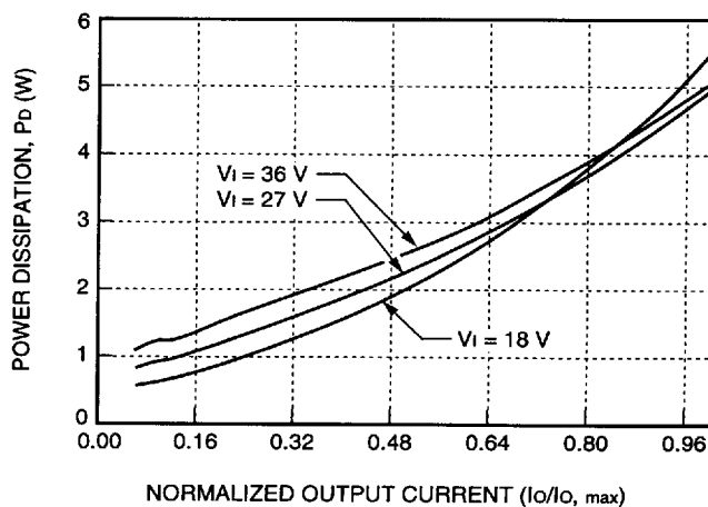
Figure 47. LC015B, C Typical Power Dissipation vs. Normalized Output Current at T_c = 25^\circ\text{C}
