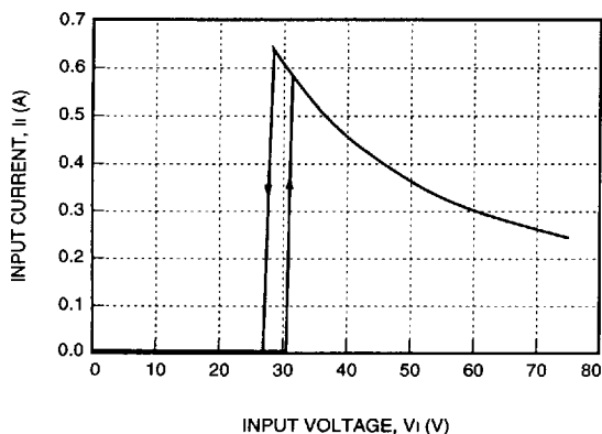
Figure 4. LW015 Input Current vs. Input Voltage at I_o = I_{o, \max} and T_c = 25^\circ\text{C}
