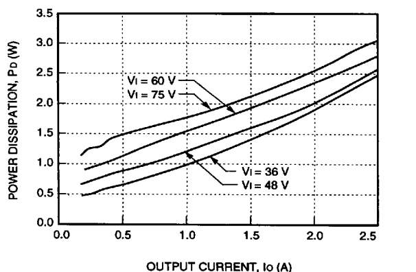
Figure 59. LW010F Typical Power Dissipation vs. Output Current at T_c = 25^\circ\text{C}
