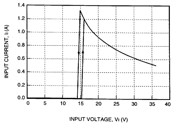
Figure 2. LC015 Input Current vs. Input Voltage at I o = I o, max and T c = 25 °C
