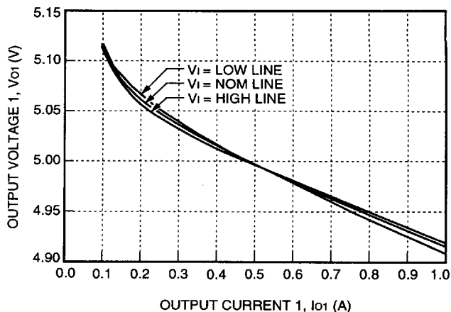
Figure 6. Lx010AJ Typical Load Regulation of Output1 with Fixed I_{o2} = 0.5\text{ A} at T_c = 25^\circ\text{C}
