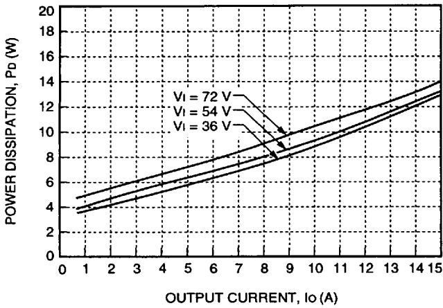
Figure 29. JW075A Power Dissipation vs. Output Current
