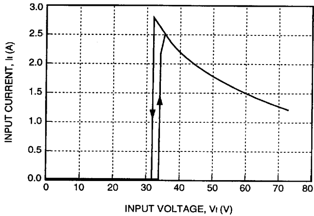
Figure 2. Typical JW075A Input Characteristics at Room Temperature, I_o = 15 A
