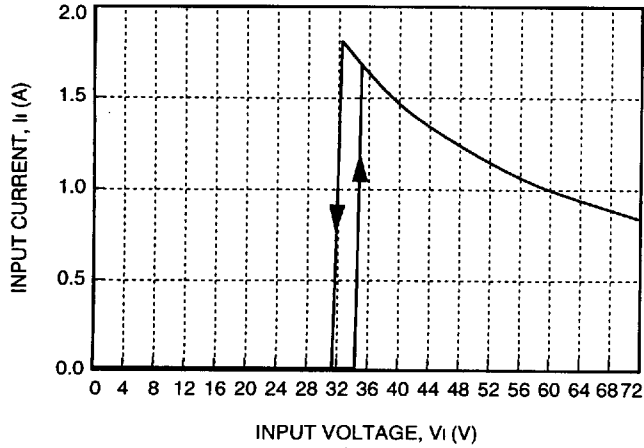
Figure 1. Typical JW050A Input Characteristics at Room Temperature, I_o = 10 A
