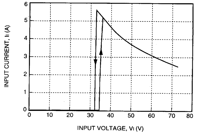
Figure 4. Typical JW150A Input Characteristics at Room Temperature, I_o = 30 A
