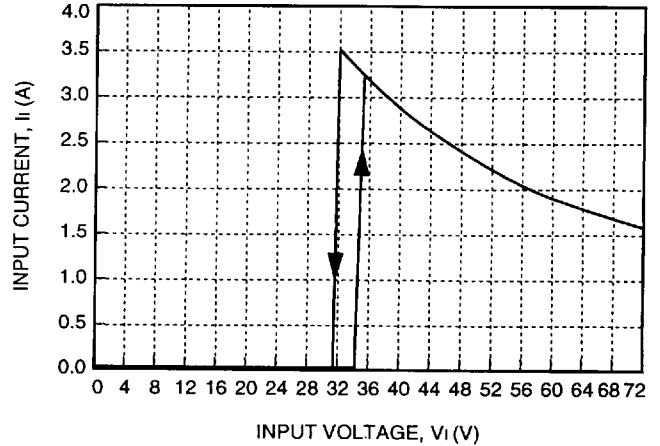
Figure 3. Typical JW100A Input Characteristics at Room Temperature, I_o = 20 A
