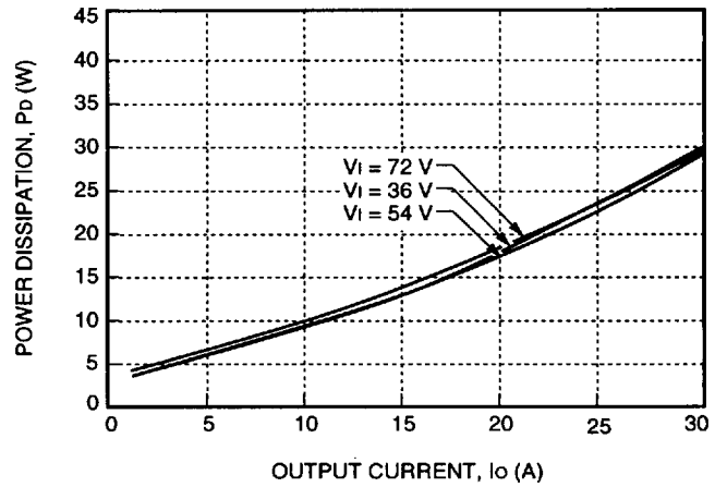
Figure 31. JW150A Power Dissipation vs. Output Current
