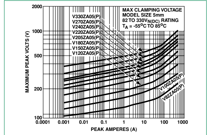
Figure 4 - V82ZA05(P) - V330ZA05(P)
