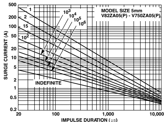
Figure 15 - V82ZA05(P) - V750ZA05(P)
