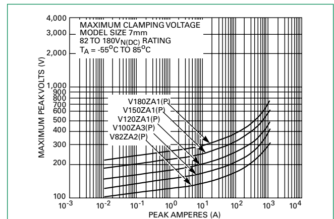
Figure 7 - V82ZA2(P) - V180ZA1(P)
