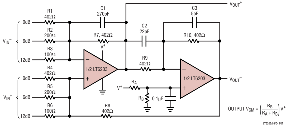
Low Noise Differential Amplifier with Gain Adjust and Common Mode Control
