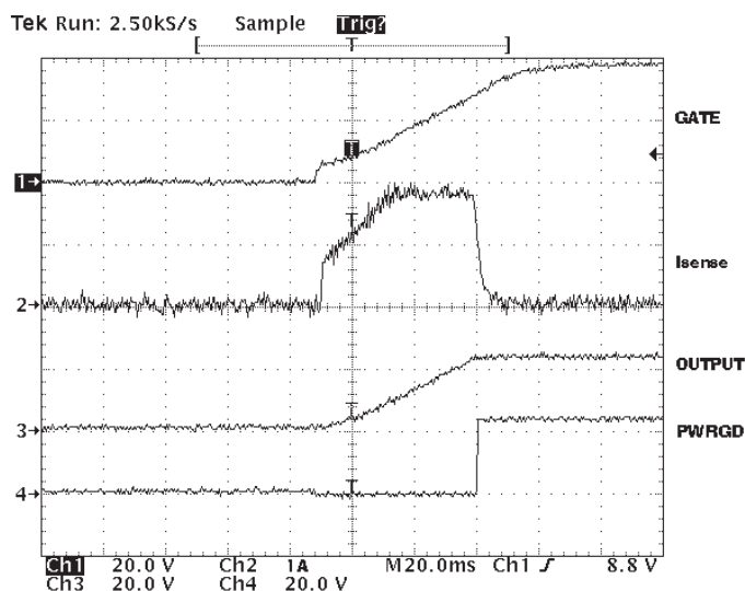
Figure 6. Power-Up Waveforms
