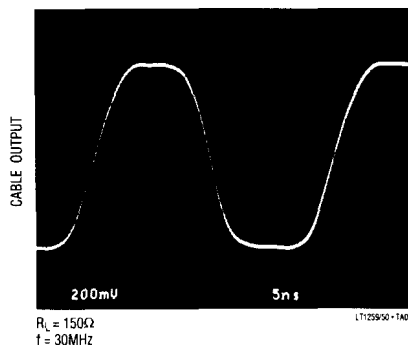
Square Wave Response
