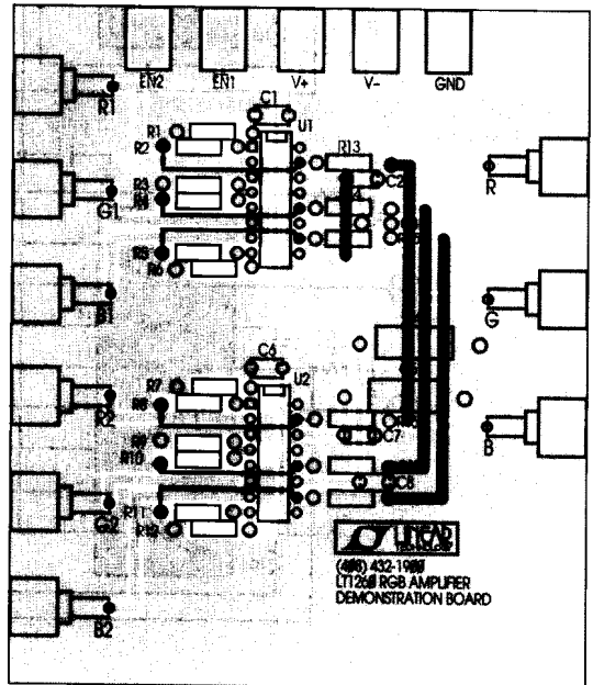
P-DIP PC Board #039
