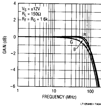
RGB Demo Board Gain vs Frequency
