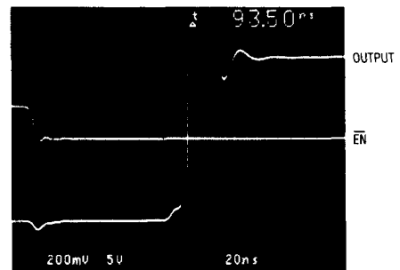
Amplifier Enable Time, A_V = 10
