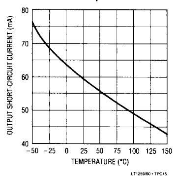
Output Short-Circuit Current vs Junction Temperature
