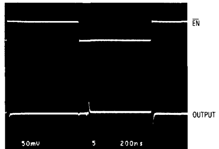
Output Switching Transient
