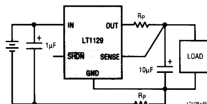
Figure 1. Kelvin Sense Connection
