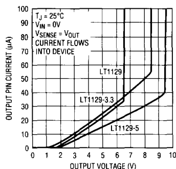
Figure 3. Reverse Output Current
