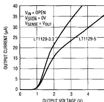
Figure 5. Reverse Output Current
