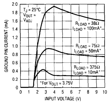
LT1129 Ground Pin Current
