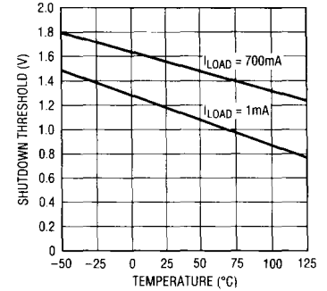
Shutdown Pin Threshold (Off-to-On)
