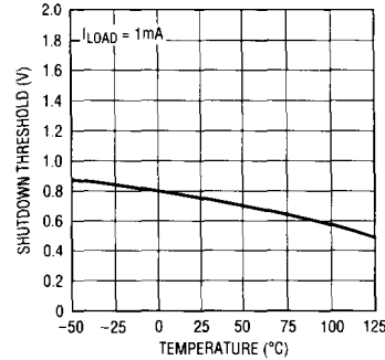
Shutdown Pin Threshold (On-to-Off)
