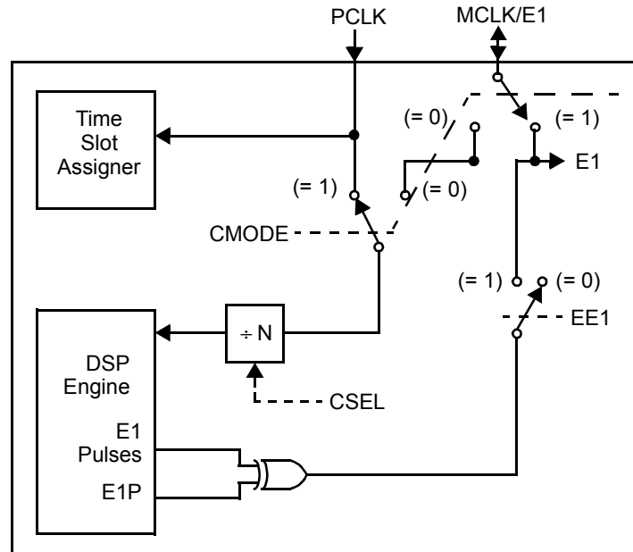
Figure 16. Clock Mode Options.
