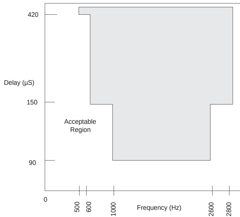
Figure 3. Group Delay Distortion
