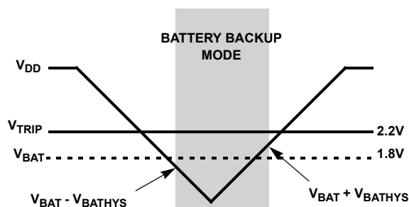
FIGURE 9. BATTERY SWITCHOVER WHEN V_{\text{BAT}} < V_{\text{TRIP}}
