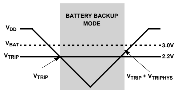
FIGURE 10. BATTERY SWITCHOVER WHEN V_{\text{BAT}} > V_{\text{TRIP}}
