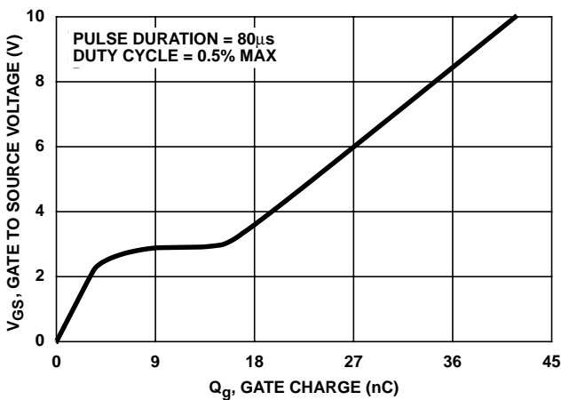
FIGURE 5. GATE TO SOURCE VOLTAGE vs GATE CHARGE
