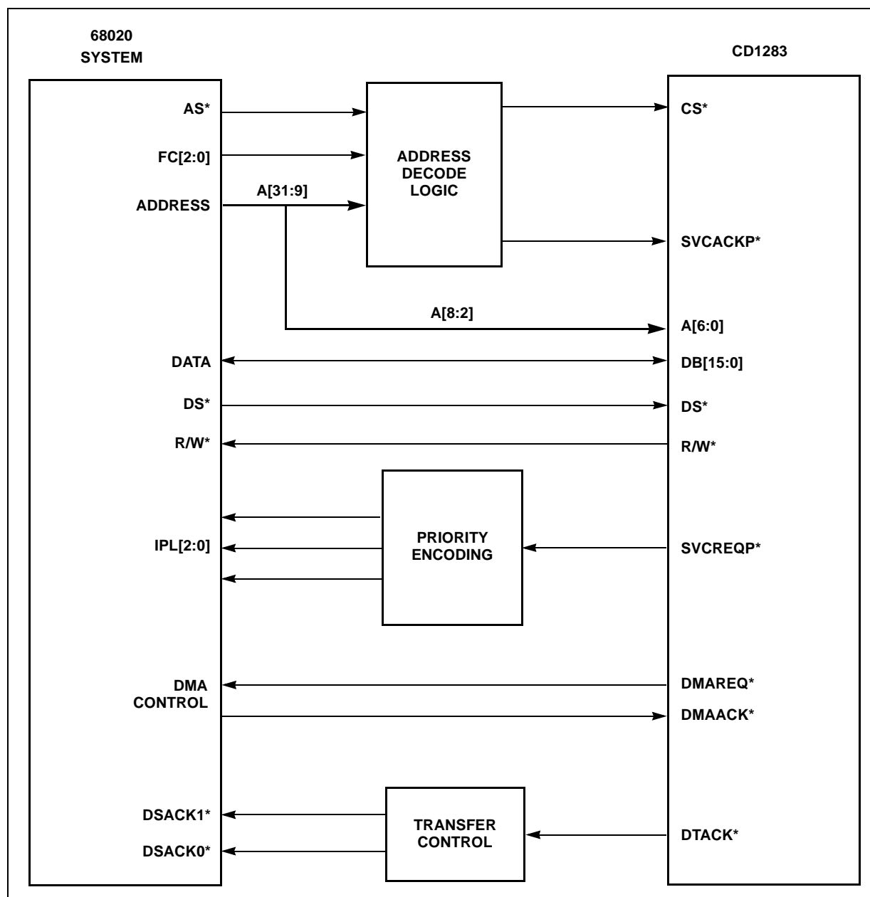
Figure 14. Motorola® 68020 Interface
