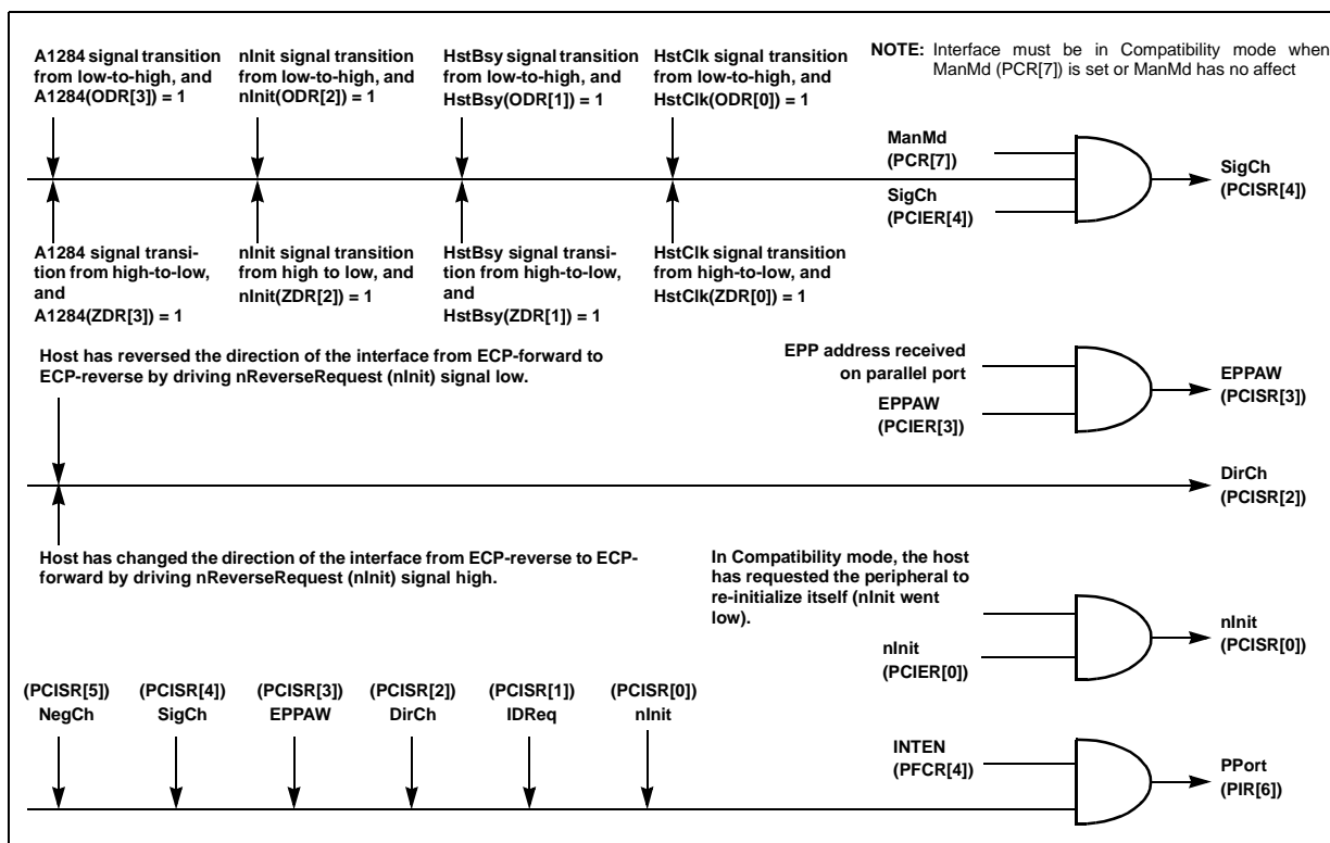
Figure 5. Interrupt Generation Logic (Continued)
