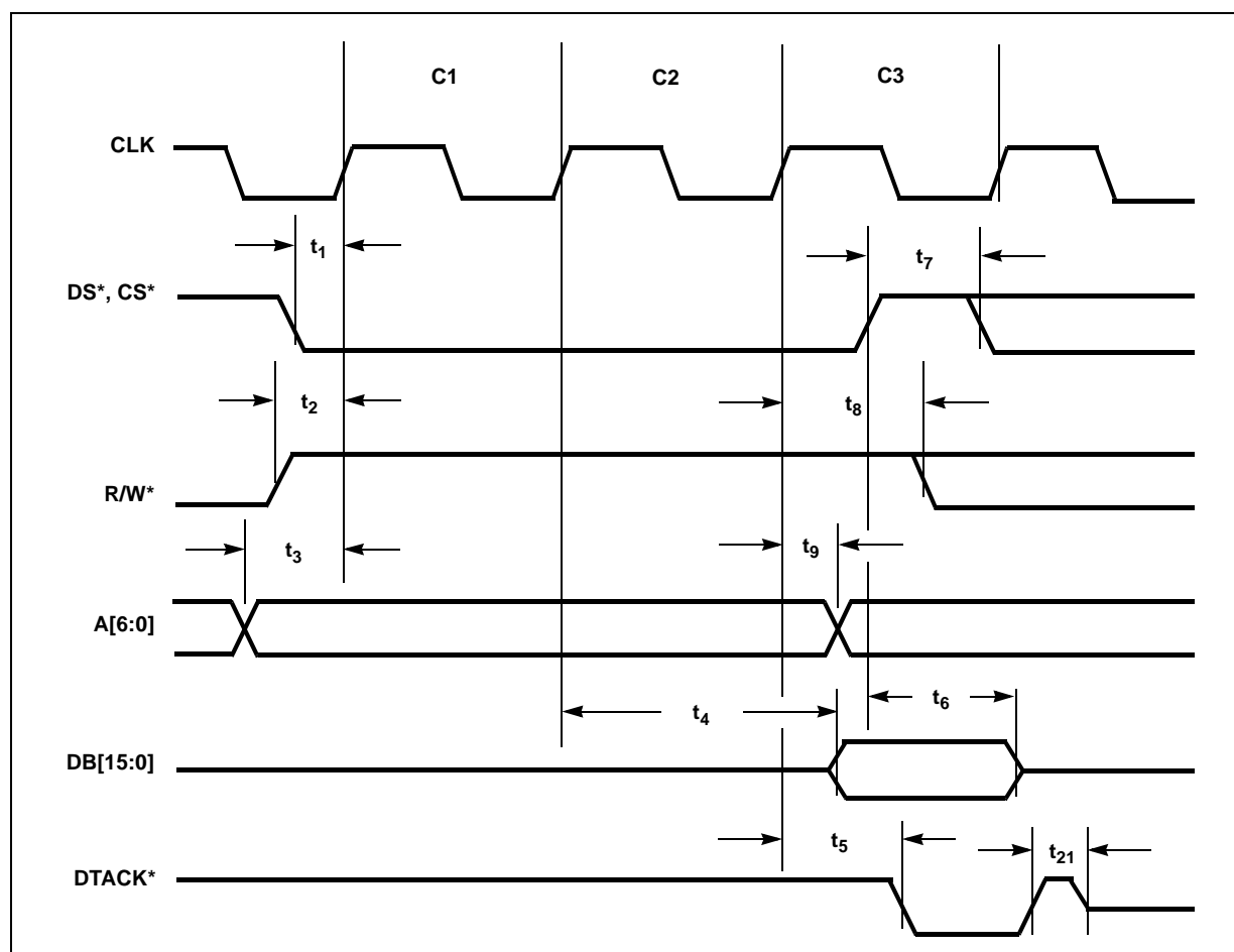
Figure 26. Synchronous Read Cycle Timing
