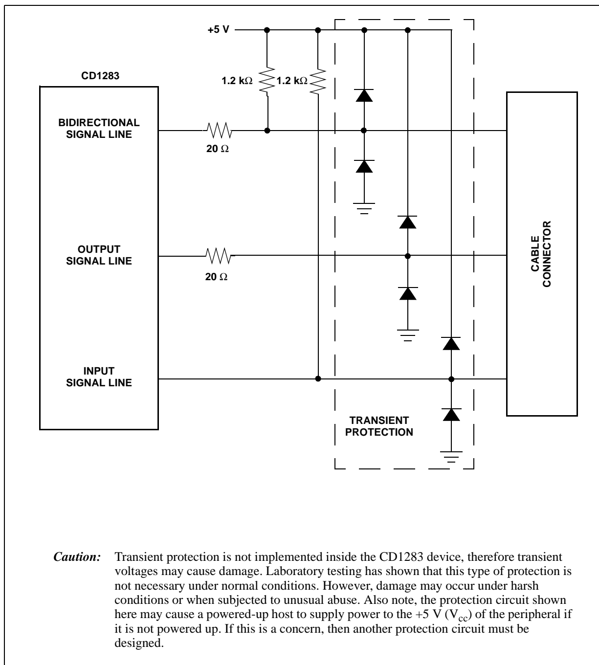
Figure 10. Cable Connection
