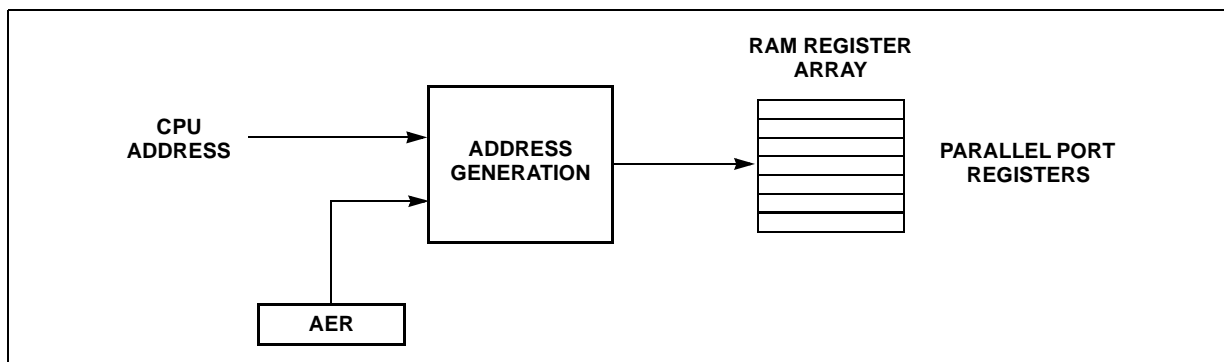
Figure 3. Internal Address Generation
