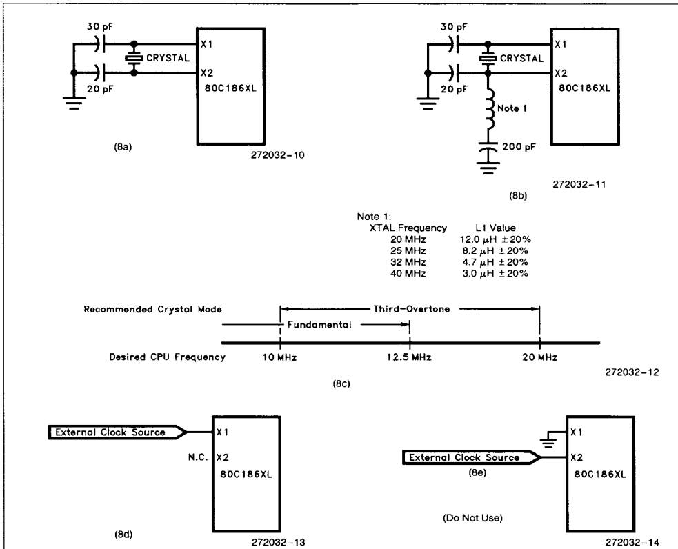
Figure 8. 80C186XL Oscillator Configurations (see text)
