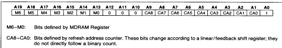
Figure 41. Addresses Generated by RCU
