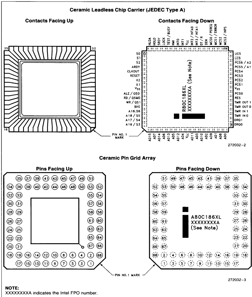
Figure 2. 80C186XL Pinout Diagrams
