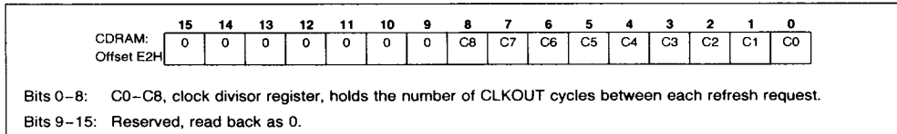
Figure 42. Clock Pre-Scaler Register
