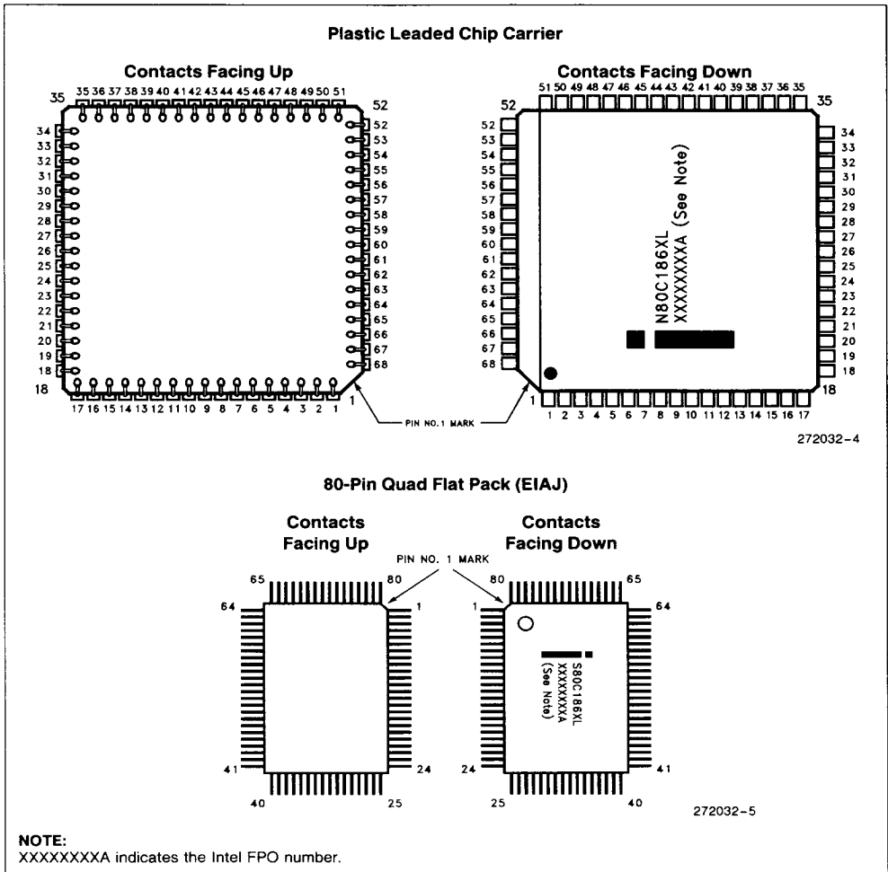
Figure 2. 80C186XL Pinout Diagrams (Continued)
