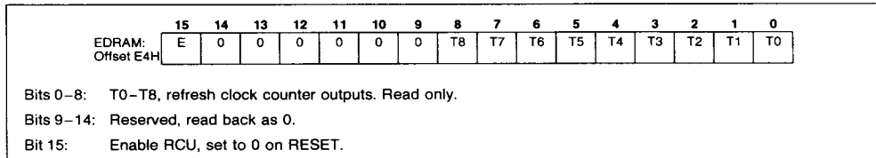
Figure 43. Enable RCU Register
