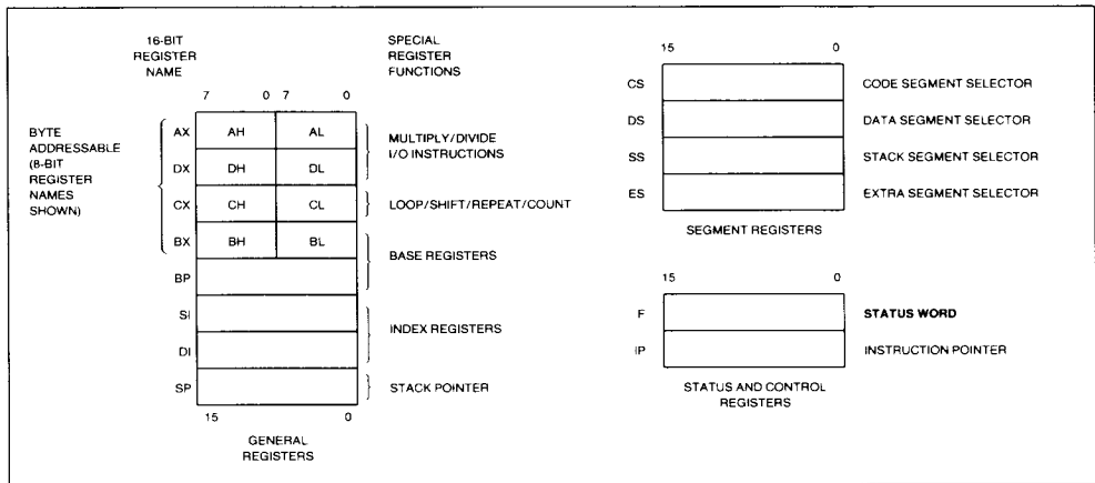
Figure 3a. 80C186XL Register Set
