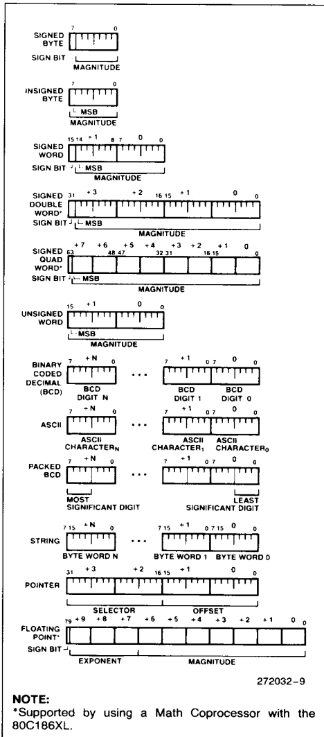
Figure 7. 80C186XL Supported Data Types
