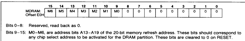
Figure 40. Memory Partition Register
