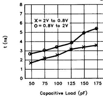
Figure 48. TTL Level Rise and Fall Times for Output Buffers
