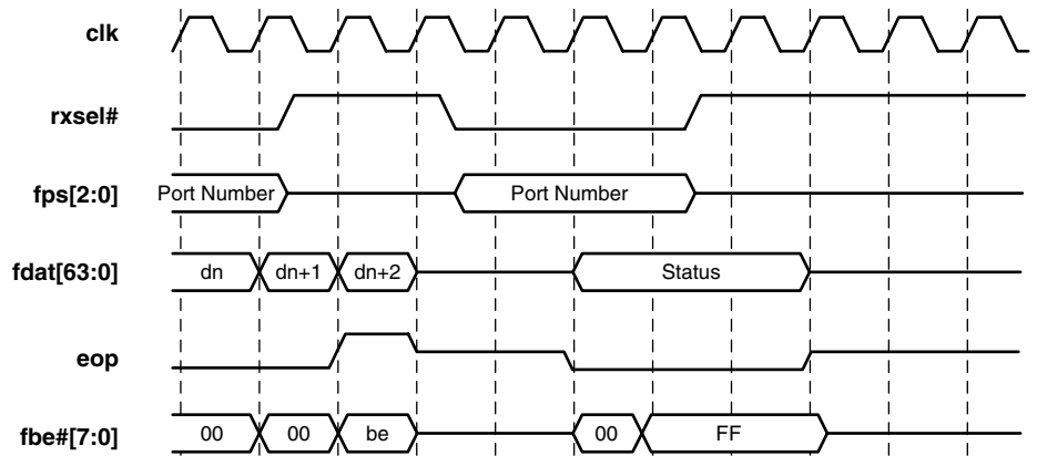
Figure 10. Fastest Receive Reaccess After EOP
