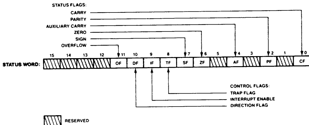
Figure 3. Status Word Format
