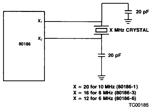
Figure 8. Recommended 80186 Crystal Configuration
