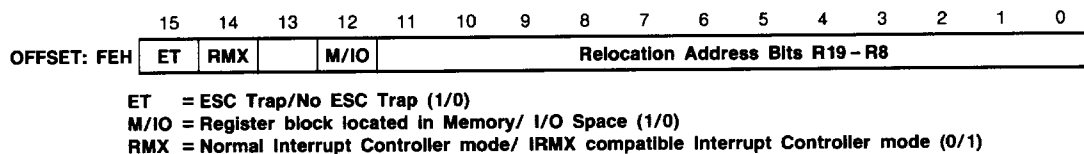
Figure 9. Relocation Register
