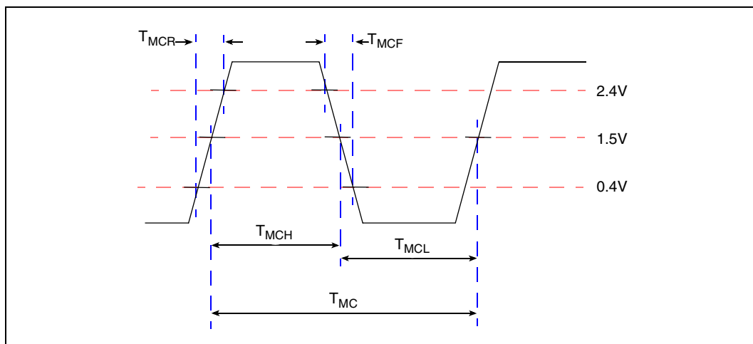
Figure 7. MCLK Waveform
