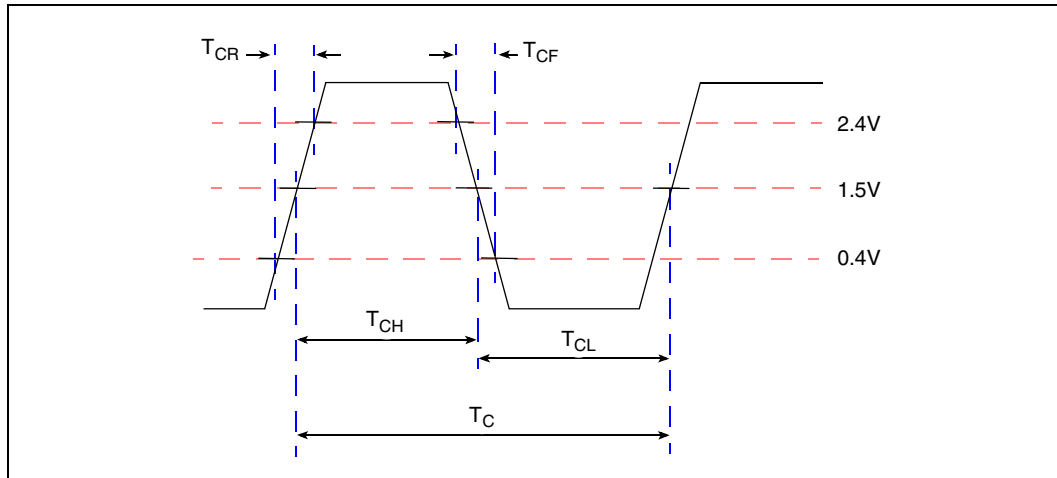
Figure 7. MCLK Waveform
