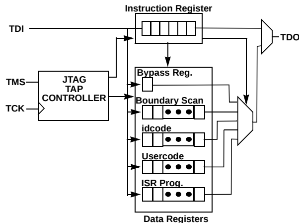
Figure 6. JTAG Interface
