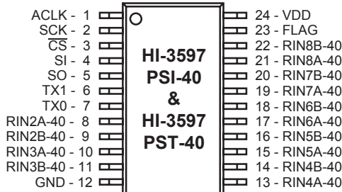
24 - Pin Plastic Small Outline Package (SOIC)
