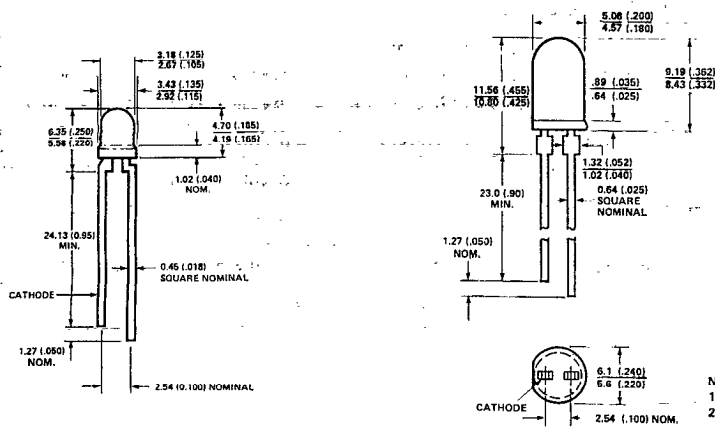
Figure A. T-1 Package.
