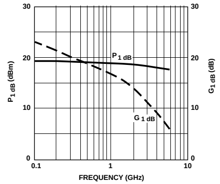
Figure 3. ATF-21186 Power Output at 1 dB Compression and 1 dB Compressed Gain vs. Frequency. V_{DS} = 3\text{ V} , I_{DS} = 70\text{ mA} .
